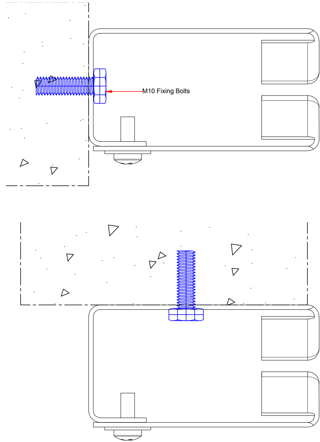
01 Guide Fixing Options 101 Elevation, Plan & Section Scale 1:1
