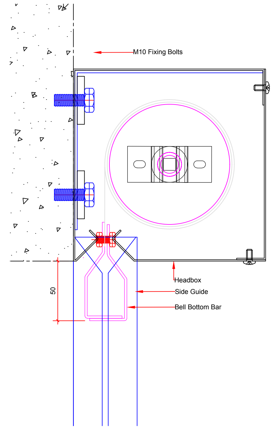
02 Section detail 101 Scale 1:2
