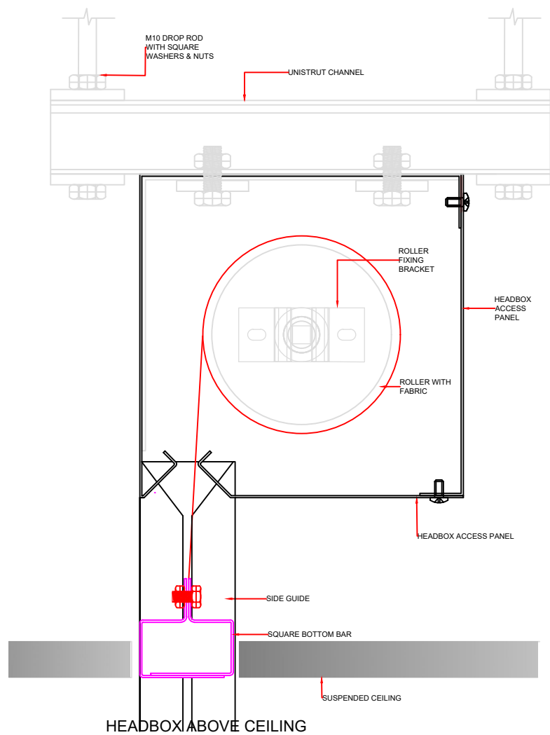
HEADBOX ABOVE CEILING
